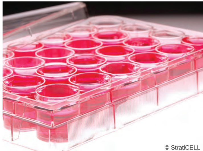
Tests d'objectivation in vitro
